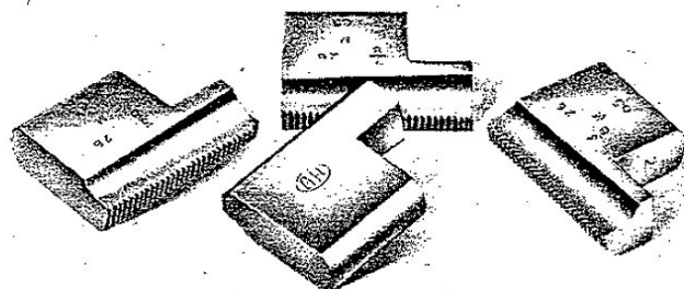
Fig. 33. A set of dies for use in a Herbert Solid Adjustable Diehead
