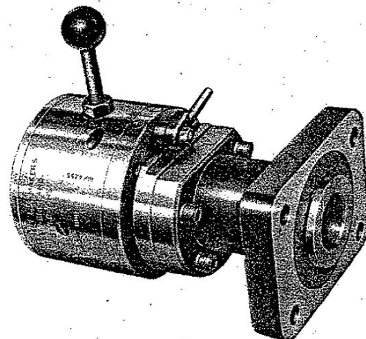
Fig. 10. C.H.S. Diehead with Flanged Adaptor
