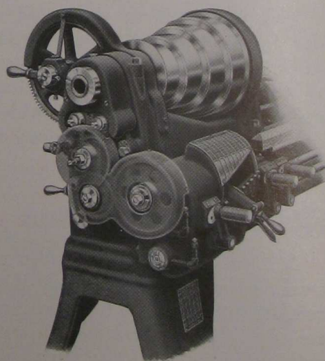
Metric transposing gears in place (Fig. No. 2)
