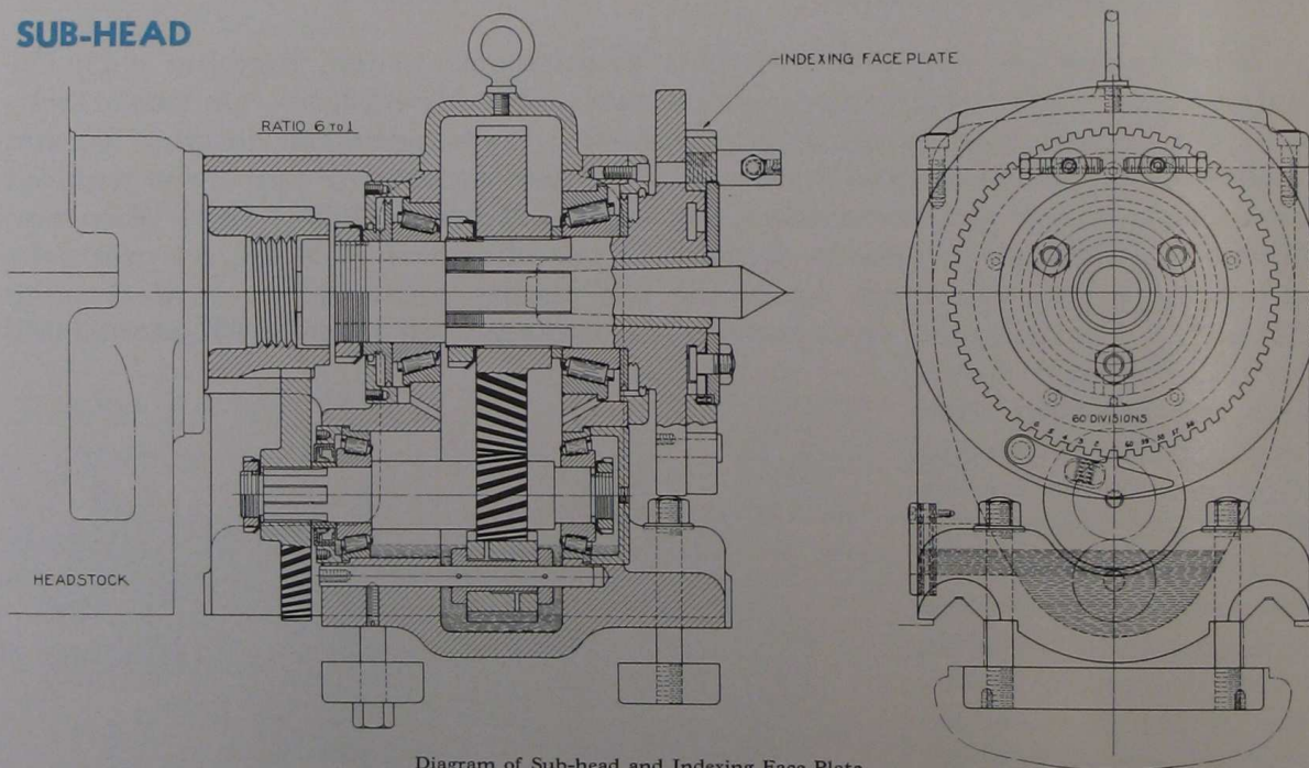
Diagram of Sub-head and Indexing Face Plate.
