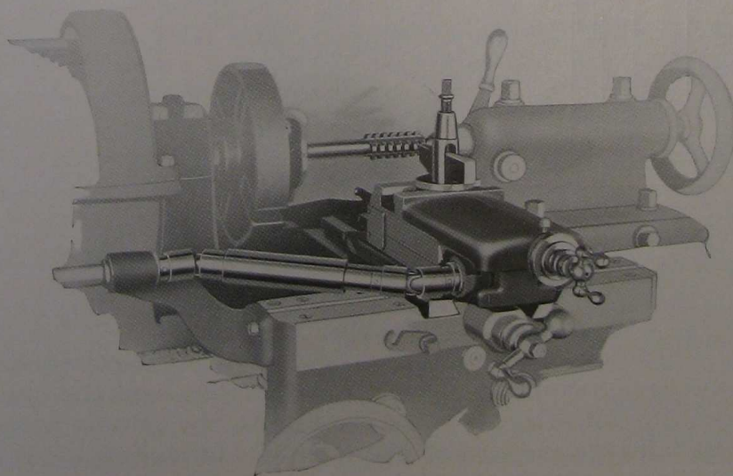
Cylindrical relief
