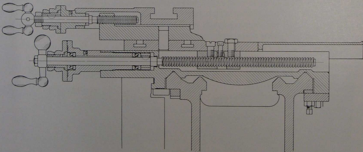
Carriage Assembly with Anti-friction Cross Feed Screw and Compensating Nut (Fig. No. 3)
