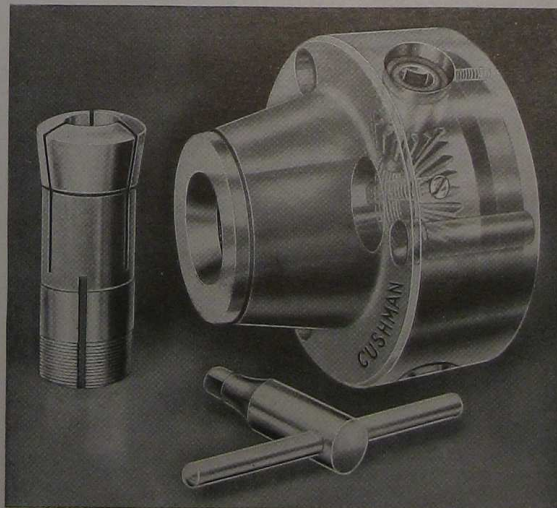
Nose-type collet chuck (Fig. No. 2)
