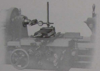
Testing cross slide alignment (Fig. No. 1)
