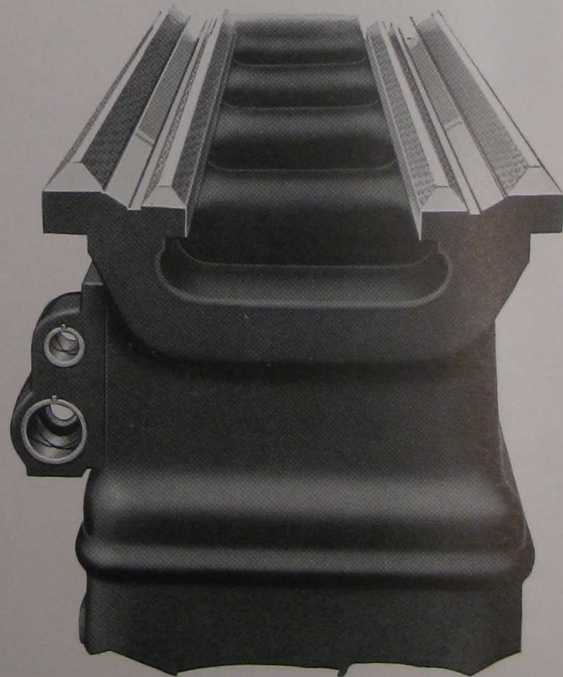
4-Vee Bed
