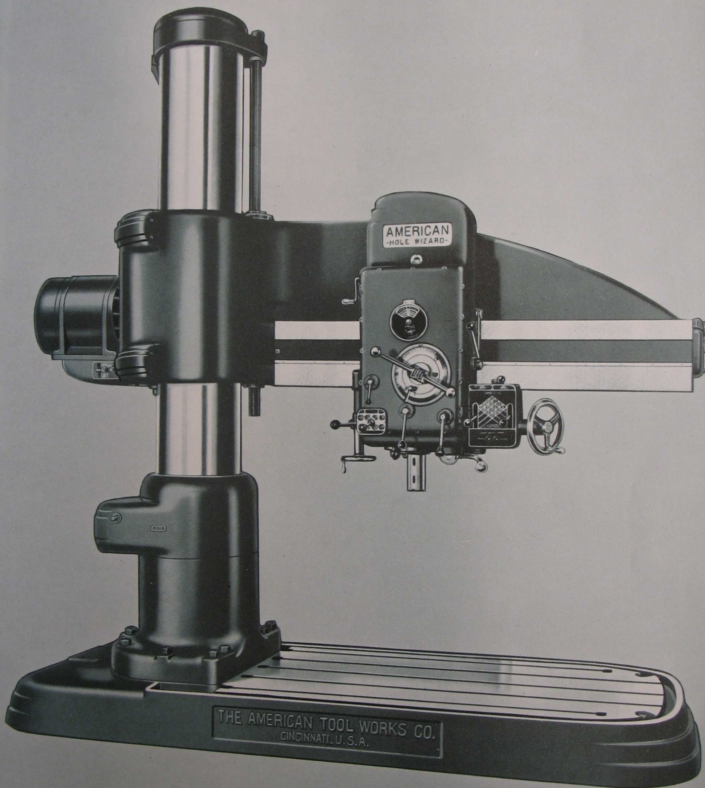
5-foot Arm, 6-foot Arm and 7-foot Arm 17-inch Column "American" Hole Wizard Radial. Descriptive Bulletin No. 327.
