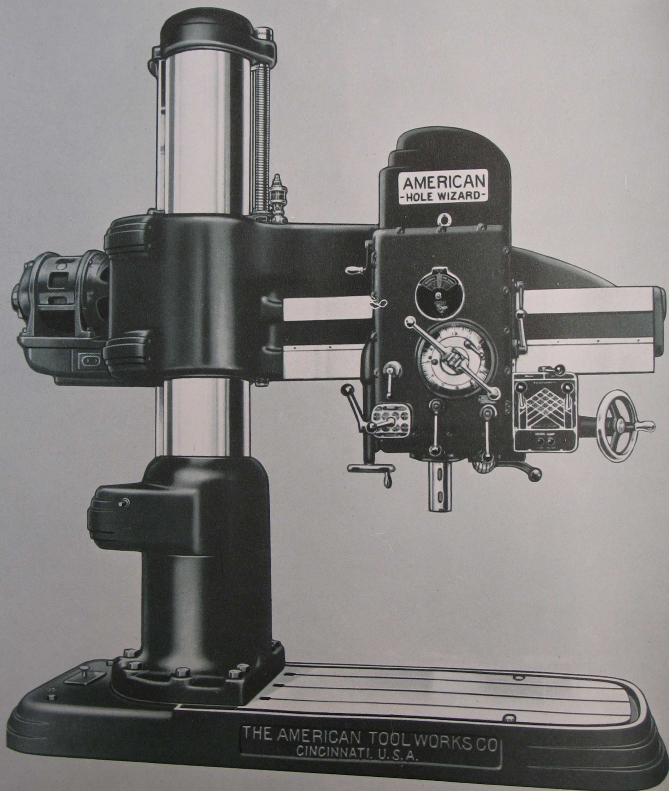
4-foot Arm, 5-foot Arm and 6-foot Arm 13-inch and 15-inch Column "American" Hole Wizard Radial. Descriptive Bulletin No. 327.
