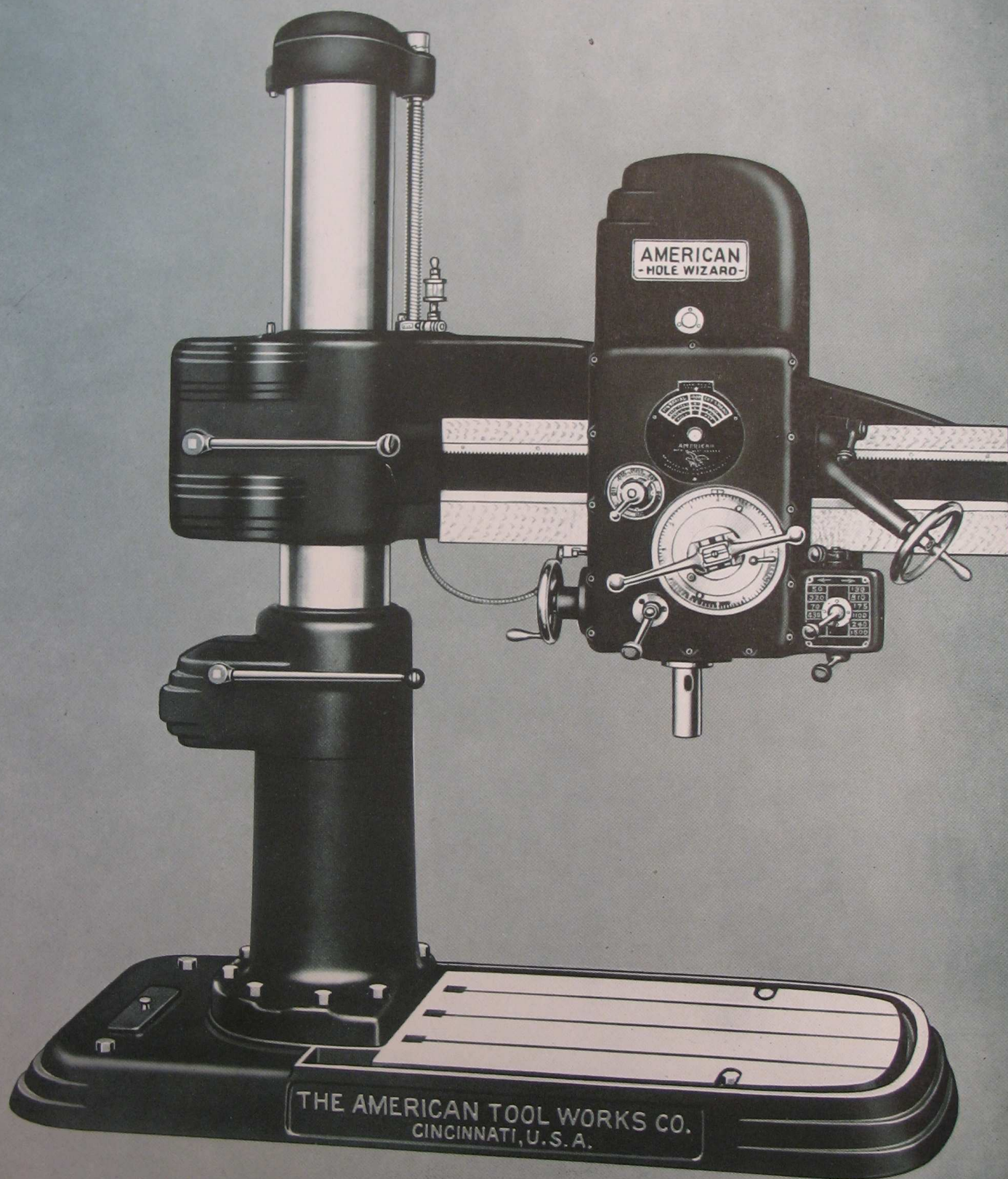
3-foot Arm, 9-inch Column "American" Hole Wizard Radial. Descriptive Bulletin No. 310.
