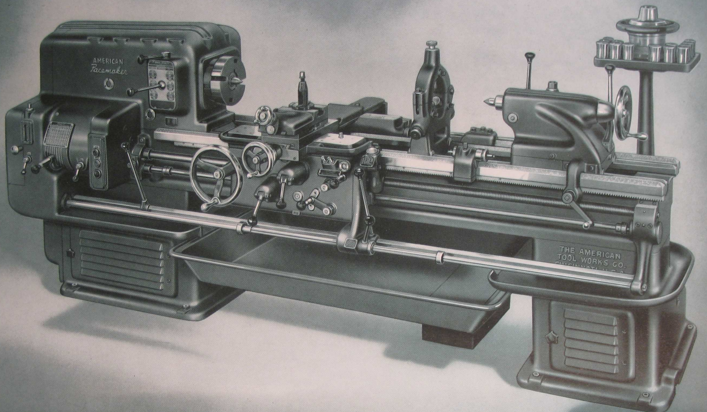
14-inch, 16-inch, 20-inch and 22-inch "American" Pacemaker Precision Tool Room Lathe. Descriptive Bulletin No. 10.
