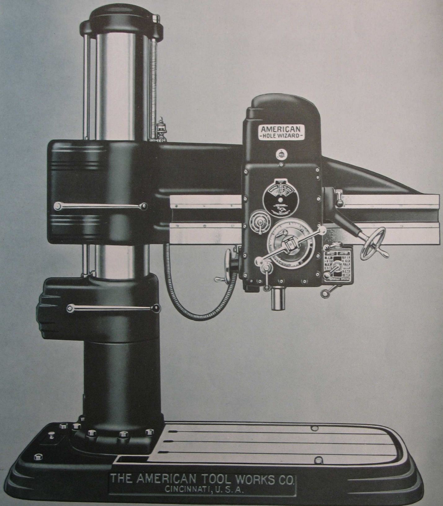
4-foot Arm, 11-inch Column "American" Hole Wizard Radial. Descriptive Bulletin No. 315.
