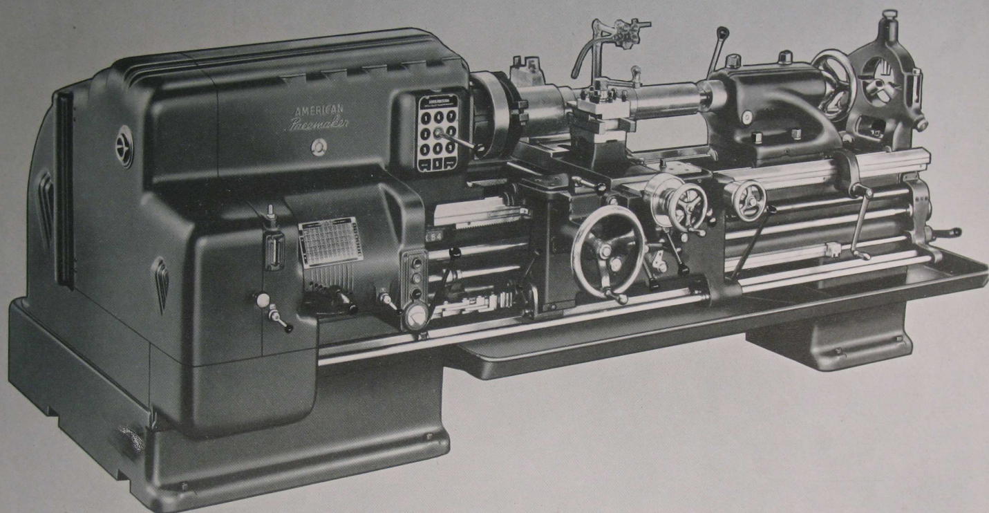
"American" Multi-Production Lathe (Pacemaker Model) with duplicating equipment (end view). Descriptive Bulletin No. 19.
