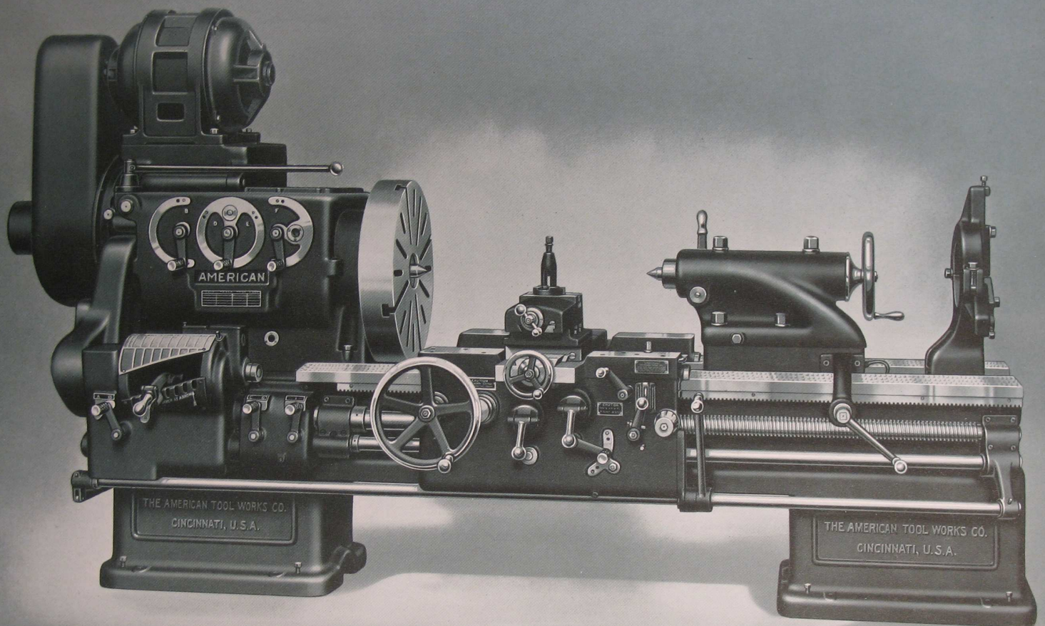
25-inch "American" High Duty Lathe. Descriptive Bulletin No. 22.
