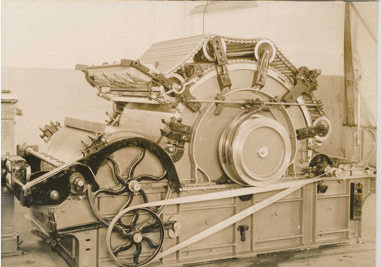
Fay & Scott, Dexter ME (Slide # 48, Image # 13-97, Collection [Products - machinery], tstamp [Thu Sep 13 14:52:09 EDT 2012]) No annotations
