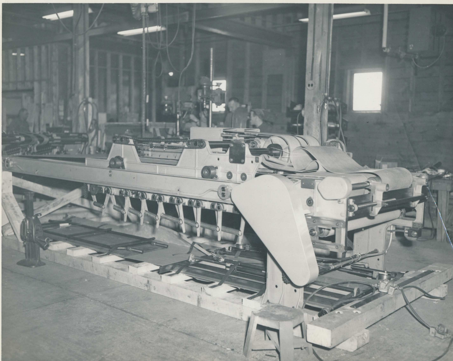
Fay & Scott, Dexter ME (Slide # 9, Image # 13108, Collection [Products - machinery], tstamp [Thu Sep 13 14:24:30 EDT 2012]) No annotations
