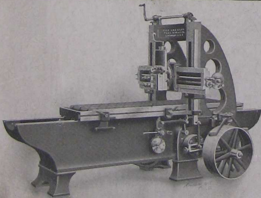
The New "American" Planer
