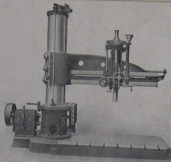
The New "American" Radial.
