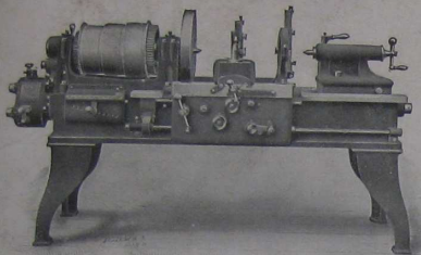
The New "American" High-Speed Lathe. For use with Special High-Speed Steels.
