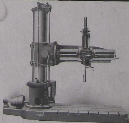
The New "American" Radial
